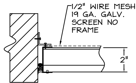
BOX FRAME
