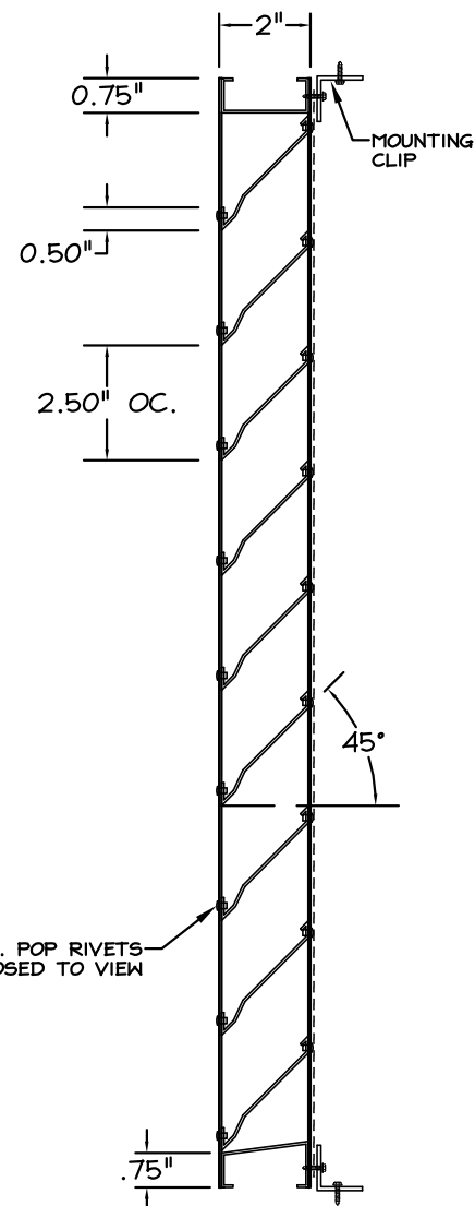
VERTICAL SECTION
